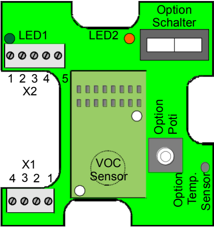
Abb. 12: Platine
